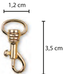
280318.. | Karabinerhaken HZ 212/13
